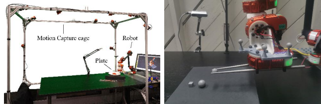
(a) Expert use teleoperation system to collect demonstrations. (b) Picking up small objects with chopsticks
